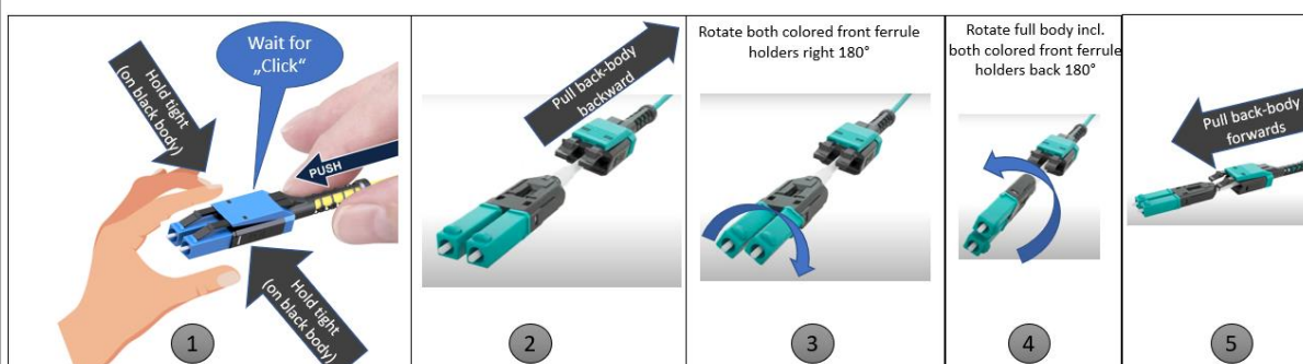
LCC-PushPull Boot
